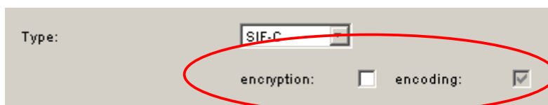
Figure 7: encryption settings
