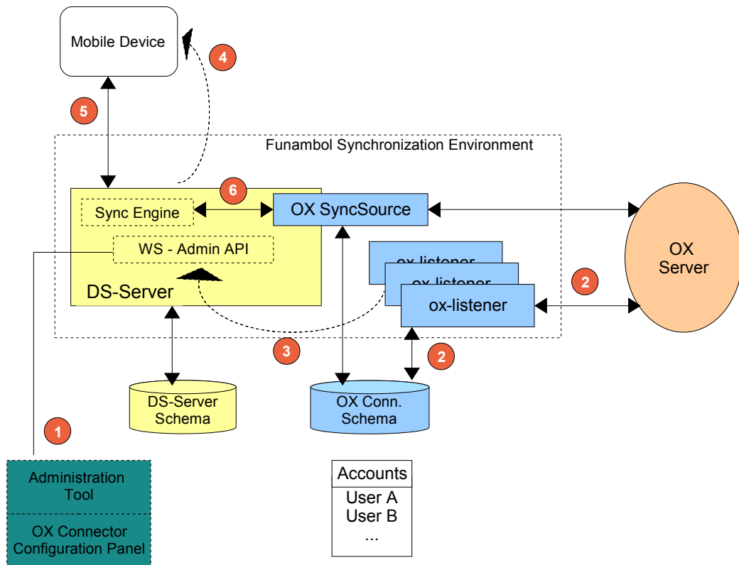
Figure 1: The Funambol ox synchronization process
