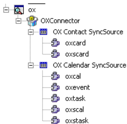
Figure 4: OX SyncSources
