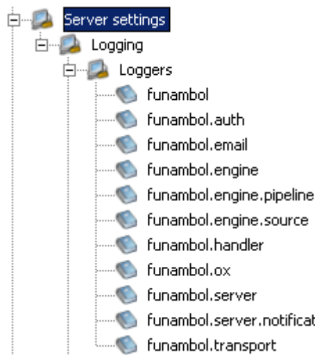
Figure 6: Logging Tree
