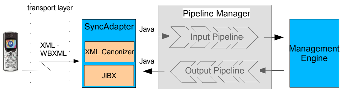
Figure 7 - Message processing architecture
