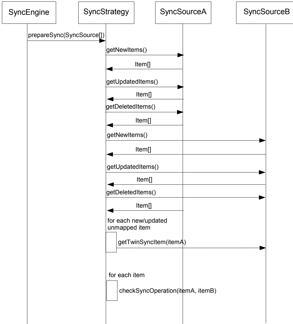
Figure 7 - Synchronization sequence diagram
